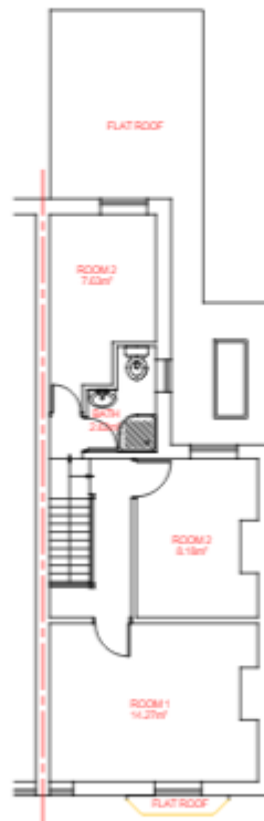
PROPOSED FLOOR PLAN FIRST SCALE 1:50
