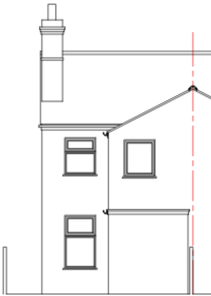
EXISTING REAR ELEVATION SCALE 1:50
